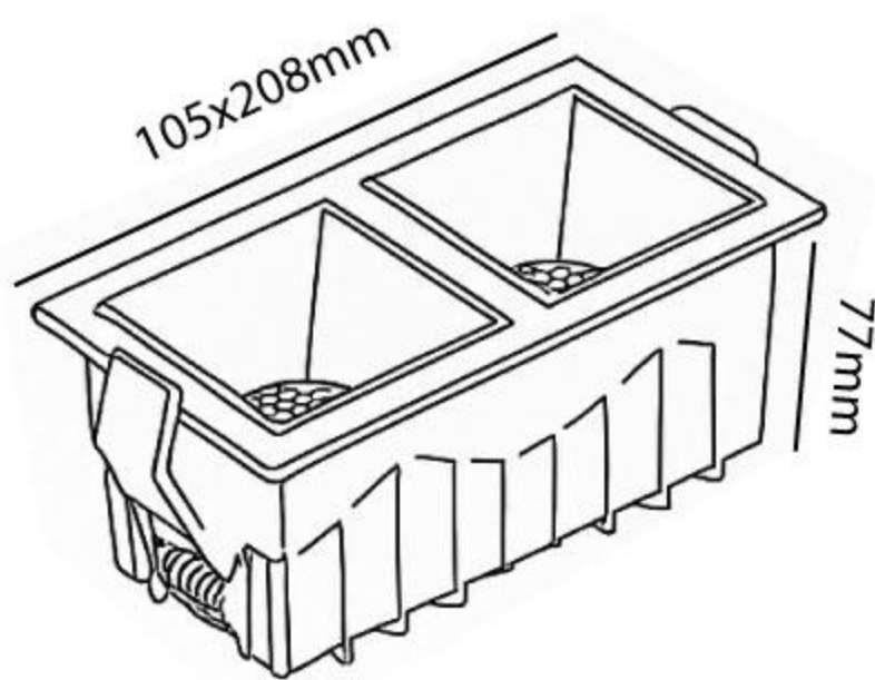
Cut-Out: 95x195mm
