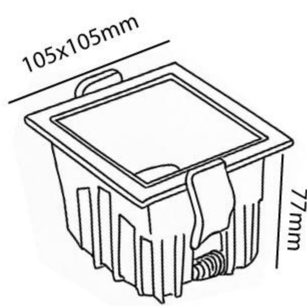
Cut-Out: 95x95mm
