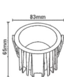
Cutout-75mm
