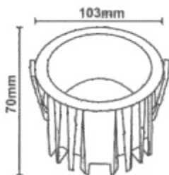
Cutout-95mm
