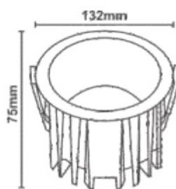
Cutout-120mm
